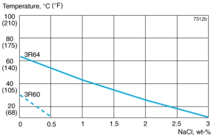
Figure 1. Crevice corrosion resistance of Sandvik 3R64 and 3R60.
